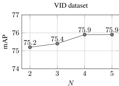
Figure 3. Detection mAP with different tubelet lengths tested on the ImageNet VID validation set without long-term information.
