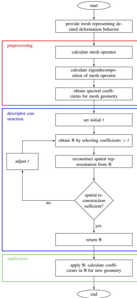
Figure 2. Exemplary workflow for finding and applying the proposed spectral shape descriptor: preprocessing (red box); construction of \mathbf{S} by selection of spectral coefficients (blue box); application of selected descriptor (green box). See main text for detailed description.
