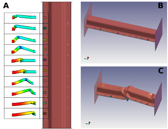
Figure 4. (A) Hat section beam used for data generation. Colored markers indicate notches introduced at various locations along the length of the shape, which lead to various different deformation behaviors shown to the left (notches denote areas of material thickness of 0.0001 mm). (B) Simulation setup with undeformed baseline shape. (C) Exemplary final time step of simulation run showing deformed shape.
