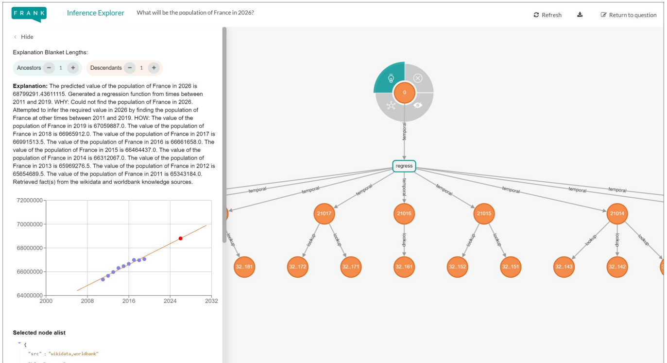
Figure 2. FRANK’s Inference Explorer showing the inference graph for the question “What will be the population of France in 2026?”. A context menu on the nodes (e.g. on node 0 above) allows users to hide or show branches and to get details of the inference nodes. The “regress” node is selected and its explanation and regression graph are displayed in the sidebar.
