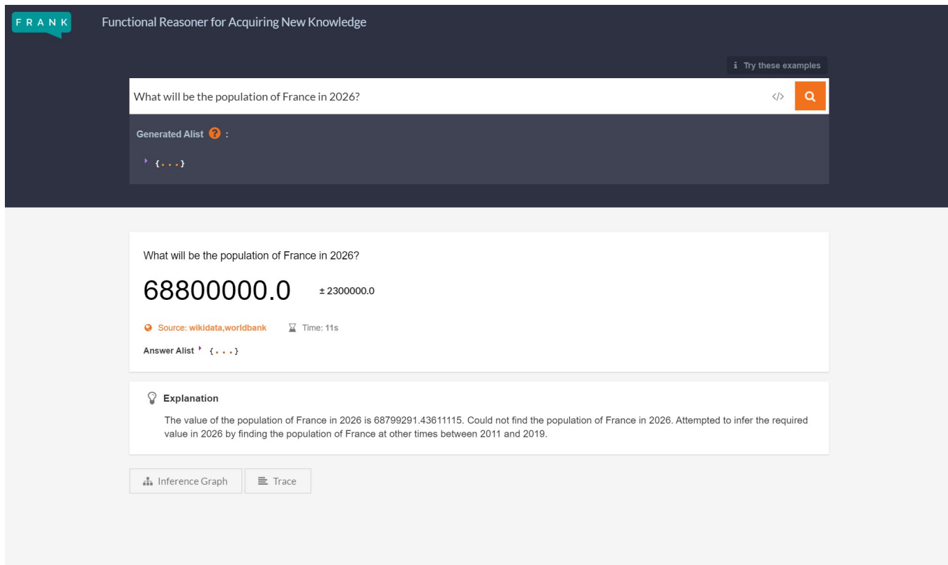
Figure 1. FRANK’s UI for the query “What will be the population of France in 2026?”
