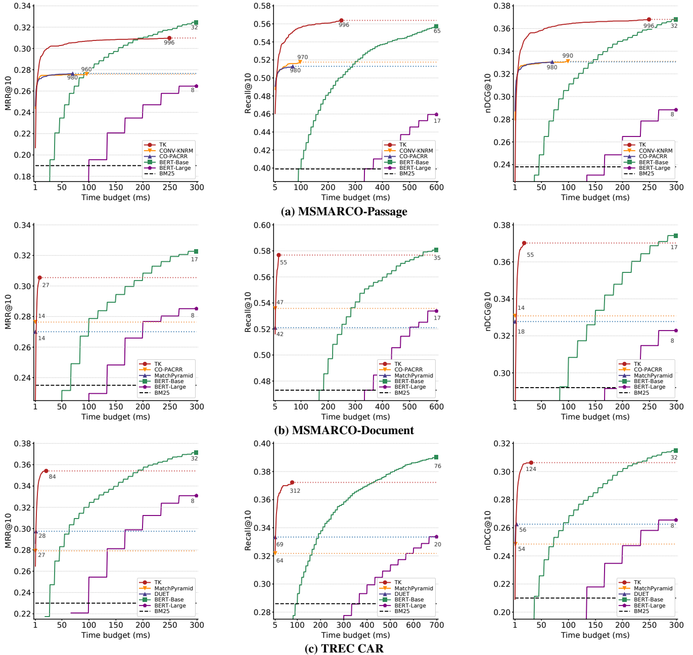
Figure 2. Time-budget analysis: We show the effectiveness (y-axis) of each model on the respective validation set by selecting the maximum number of documents to re-rank in the available time limit (x-axis). The marker indicates the best possible result; the dotted line indicates that additional time does not yield better results; the number of re-ranked documents is indicated for each best result.
