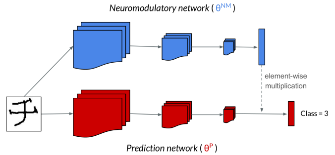
Figure 1: The architecture for A Neuromodulated Meta-Learning algorithm (ANML). The prediction network (red) is a normal neural network updated in the inner loop via SGD (or similar). The neuromodulatory network (blue) produces an element-wise gating of the prediction network’s forward-pass activations, enabling selective activation (i.e. conditional computation) and indirectly enabling selective plasticity by affecting the gradient updates of the prediction network. The initial weights (at the start of each inner loop) of both the neuromodulatory and prediction network are meta-learned in the outer-loop of optimization. The weights of the neuromodulatory network are not updated in the inner loop, but those of the prediction network are. The example image is from the Omniglot dataset, which is the experimental domain for the experiments in this paper.
